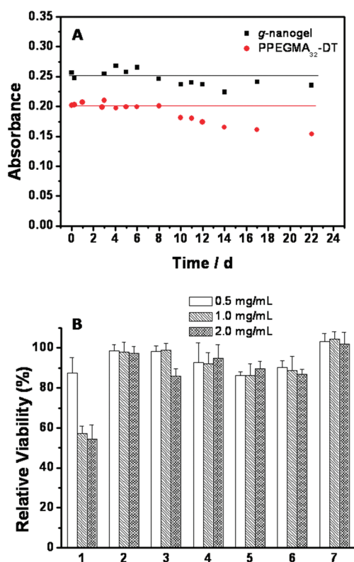
Figure 3. (A) Hydrolysis of the dithioester group in g-nanogel and PPEGMA 32 -DT in 0.1 M PBS buffer (pH = 7.4) by monitoring the UV–vis absorbance at 304 nm for g-nanogel and 307 nm for PPEGMA 32 -DT at 37 °C, [dithioester] = 0.354 mM. (The higher apparent absorbance for g-nanogel is due to scattering. Manually drawn straight lines for guidance only). (B) Cell viability of A549 cells after exposure to the polymers for 48 h at different dose of Macro-CTAs or nanogels: 1, PEGSk-TTC; 2, PPEGMA 21 -TTC; 3, PPEGMA 32 -DT; 4, l -nanogel (54 nm, entry 1, Table 1); 5, l -nanogel (56 nm, entry 2, Table 1); 6, g-nanogel (150 nm, entry 7, Table 1); 7, g-nanogel (61 nm, entry 10, Table 1).
