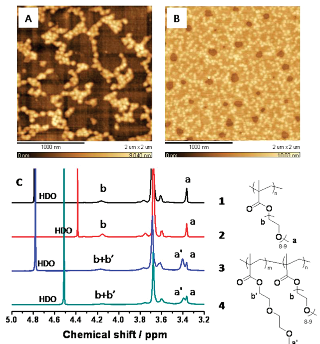
Figure 1. Atomic force microscopy (AFM) micrographs: (A) l -nanogel (entry 2, Table 1); (B) g -nanogel (entry 13). (C) Variable temperature 1 H NMR spectra in D 2 O for (1) PPEGMA 32 -DT at 22 °C, (2) PPEGMA 32 -DT at 50 °C, (3) g -nanogel (entry 9, Table 1) at 23 °C and (4) g -nanogel (entry 9, Table 1) at 40 °C. HDO peaks at different temperatures were corrected. 51
