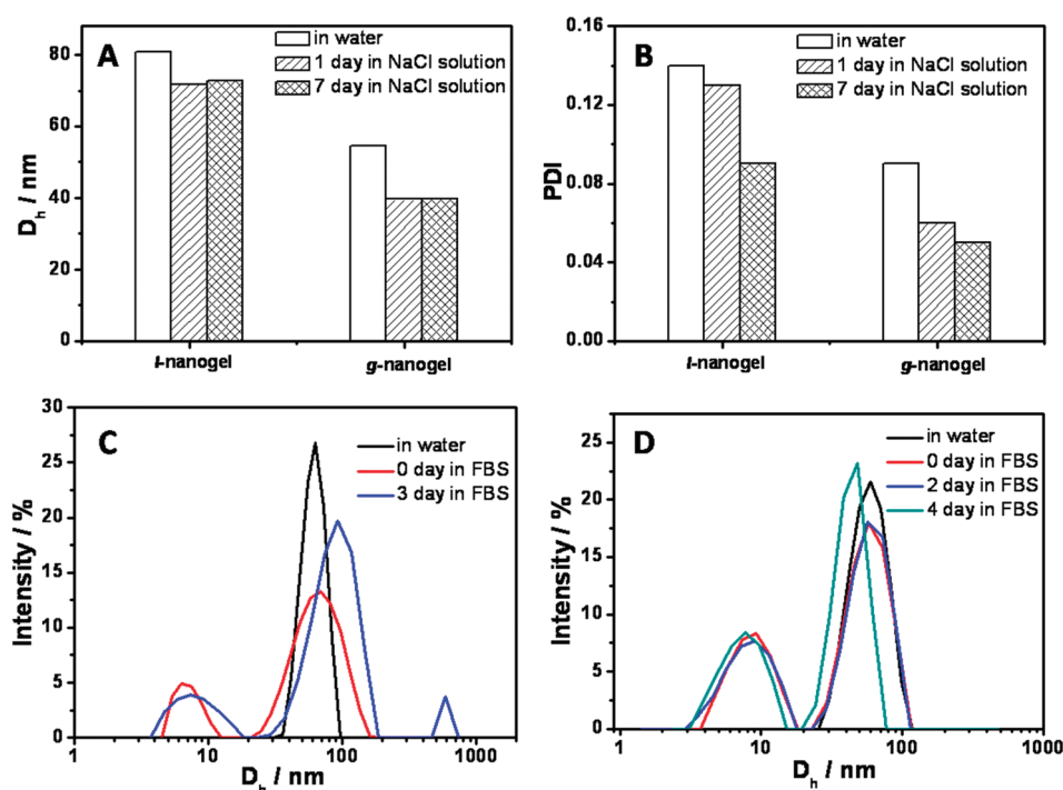
Figure 2. Dynamic light scattering (DLS) results of nanogels in NaCl solution (A and B) and FBS (C for t -nanogels and D for g -nanogels). In parts C and D, the peak below 10 nm was from FBS.
